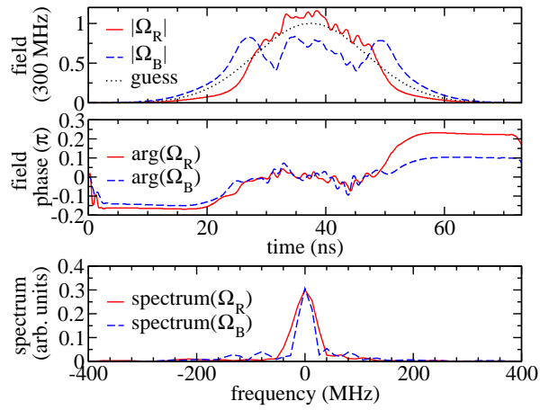
Figure 7.5: The optimized pulses resulting from optimization using two weighted states and including spontaneous decay (orange solid line in Fig. 7.2, bottom panel), using the same conventions as Fig. 7.3.
