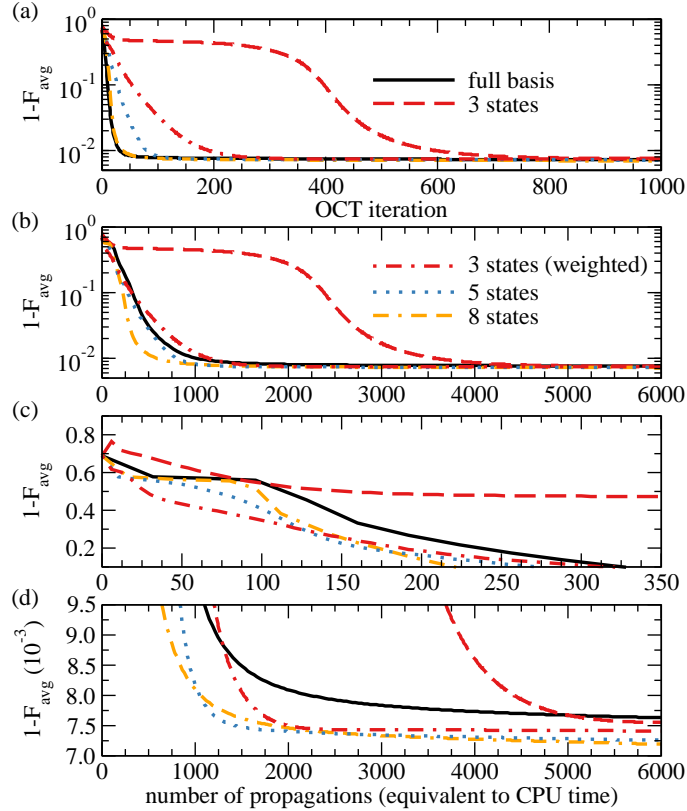
Figure 7.7: Optimizing a \sqrt{\text{iSWAP}} gate for two transmons in the presence of energy relaxation and pure dephasing (with the rates given in Table 7.2): Convergence for five choices of sets of initial states, as described in the text. The gate duration is T = 400 ns. The panels from top to bottom show the gate error over the number of iterations; the gate error over the number of state propagations, indicative of the required CPU time; a zoom on the initial phase of the optimization; and a zoom on the asymptotic convergence (panels c and d both using a linear scale).
