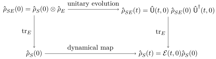
Figure 2.4: Diagram showing how the dynamical map \mathcal{E}(t, 0) is obtained by tracing out the environment from the unitary evolution of the total state. Adapted from [64].
