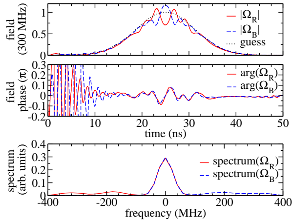
Figure 7.3: The optimized pulses \Omega_{B,R}(t) for the blue and red laser cf. Fig 7.1, resulting from optimization using two states with unequal weights without spontaneous decay (corresponding to the orange solid line in the top panel of Fig. 7.2). The pulse amplitudes are shown in the top panel, the complex phase in the center panel, and the pulse spectrum in the bottom panel. The guess pulse, indicated by the black dotted line in the top panel, is identical for both the red and the blue laser. In the spectrum, frequency 0 corresponds to the carrier frequencies of the laser pulses.
